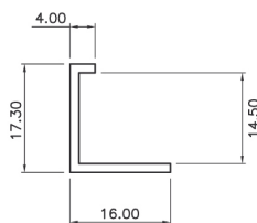
14.5mm edging 13.5mm panel
