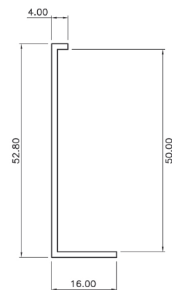
50mm edging 50mm panel
