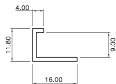
9mm edging 8mm panel
